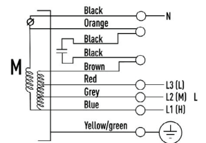
VFM190-3 B2M190-70-3 Three speed wiring
