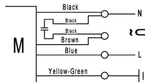
VFM190-1 B2M190-70 Single speed wiring
